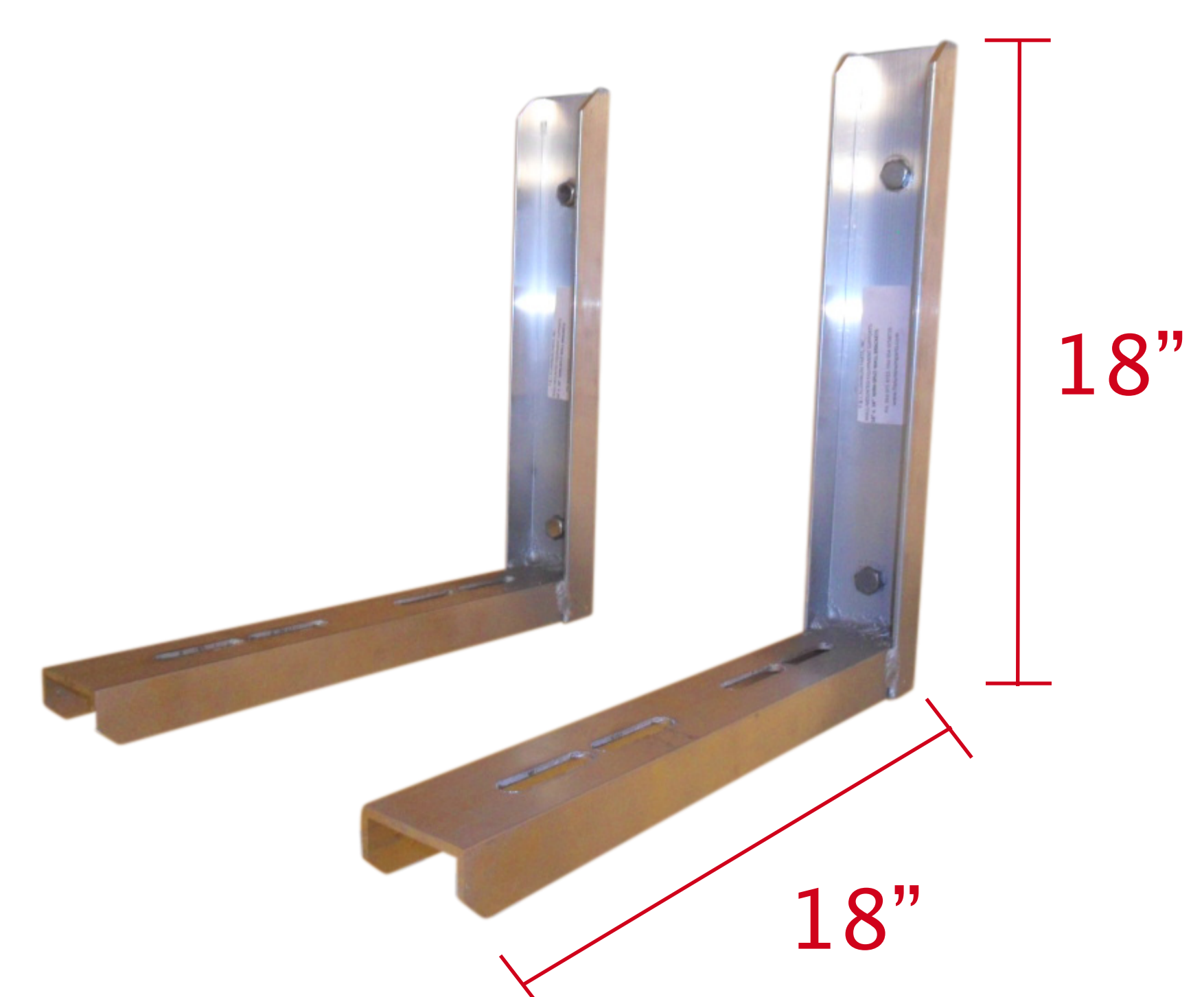
Figure 4. Mini-Split brackets
