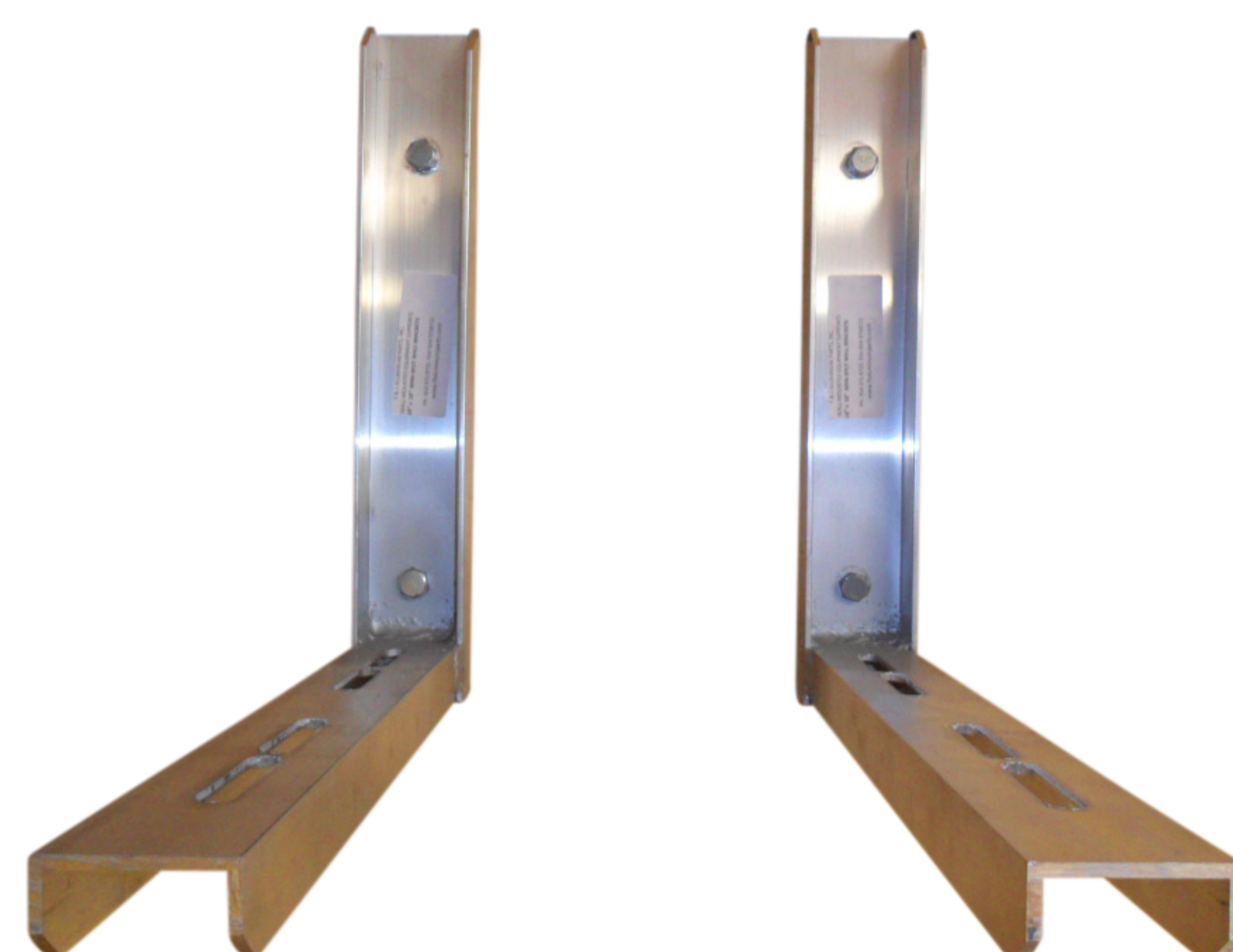
Figure 3. Mini-Split wall brackets
