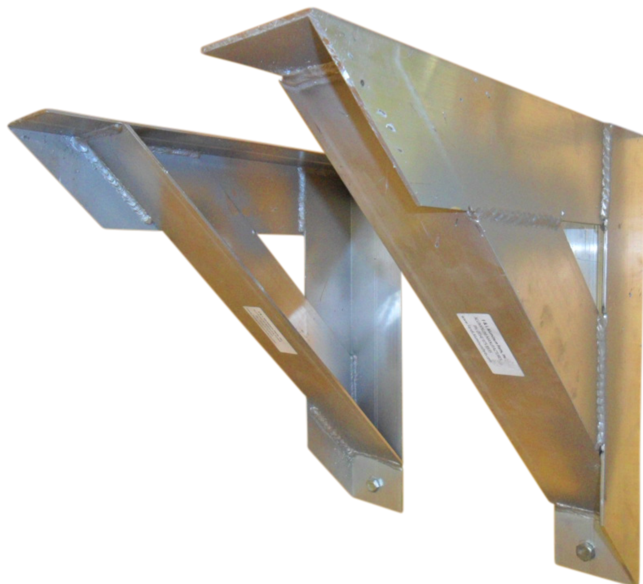
Figure 2. Pair of Wall Mounting Brackets
