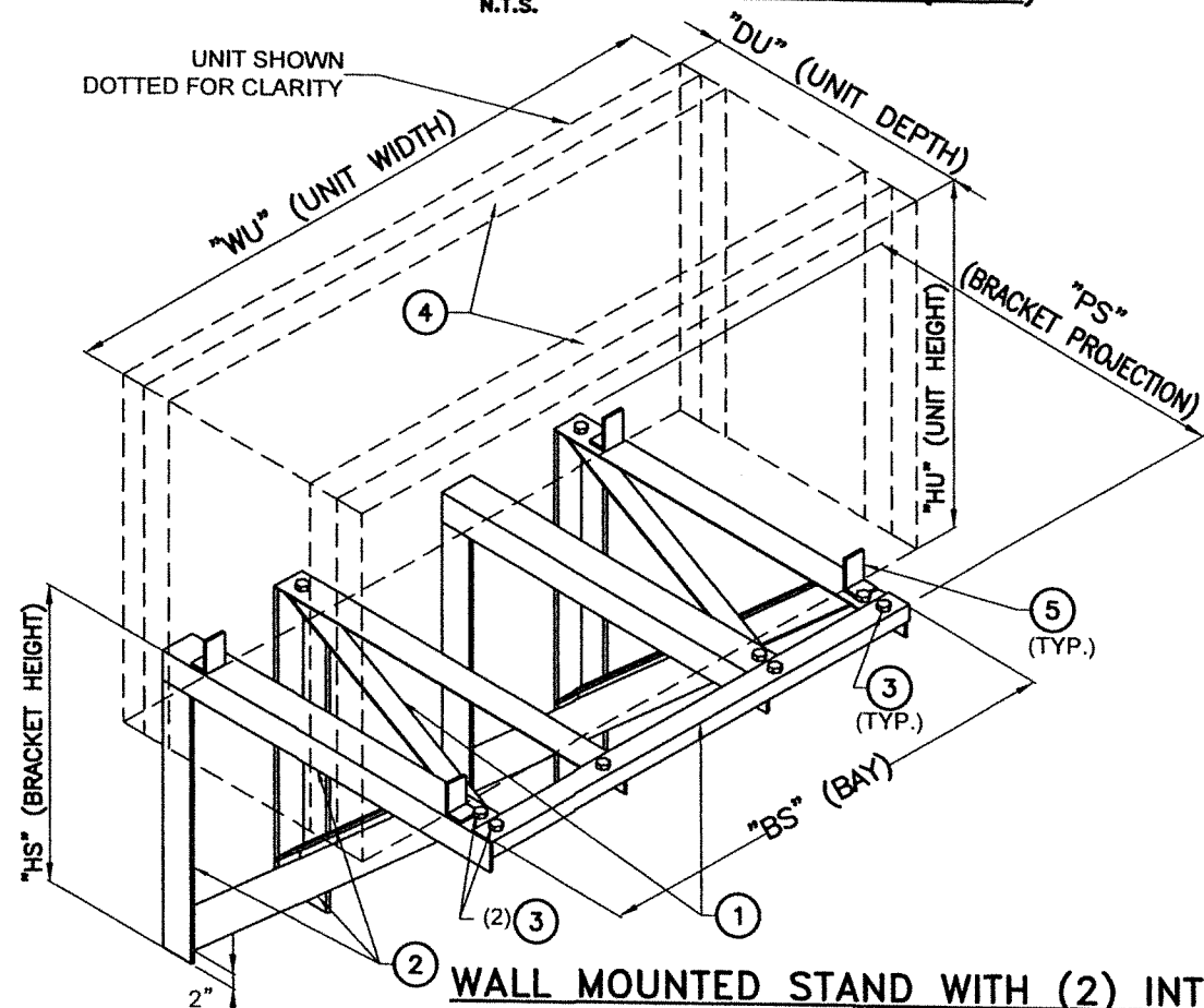
WALL MOUNTED STAND WITH (2) INTERIOR ADDITIONAL BRACKETS (PLAN) N.T.S.
