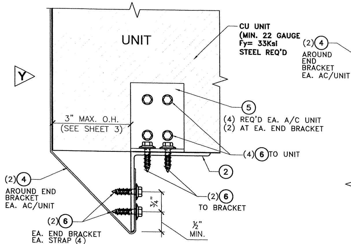
DETAIL 1 (WHEN UNIT OVERHANG) 1/2" = 0'-1" ELEVATION
